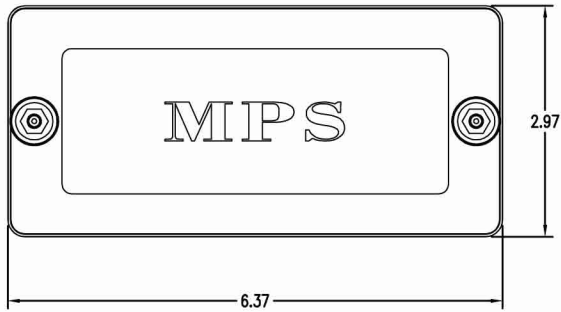
UTS1 WITH BLACK COVER
